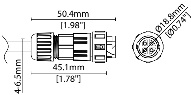
4 Pin RGB Female Connector IP67
